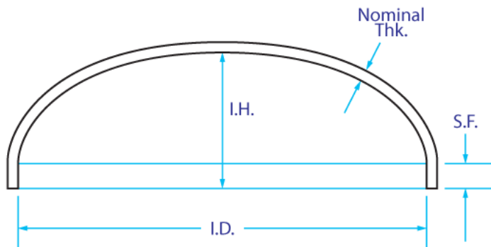
ASME • ELLIPTICAL (2:1 RATIO) Trim or bevel not shown – specify on inquiry.
