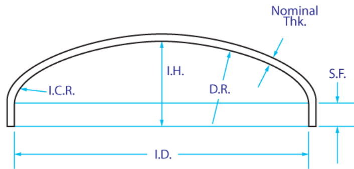
FLANGED AND DISHED Trim or bevel not shown – specify on inquiry.
